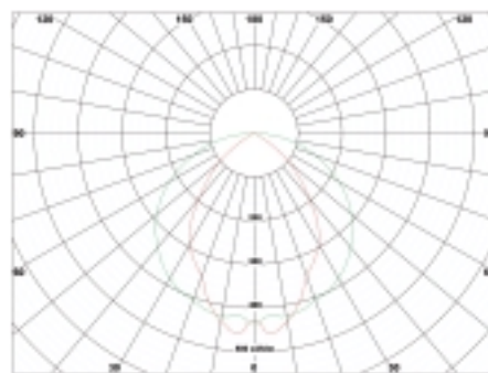
Narrow Beam Light Output ratio: 88.9%
