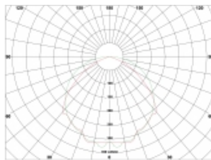
Wide Beam Light Output ratio: 89.0%
